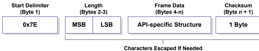
Figure 6-02. UART Data Frame Structure - with escape control characters:
